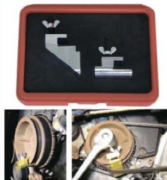
TOOL KIT FOR ELASTIC - RIBBED BELTS Universal applications
